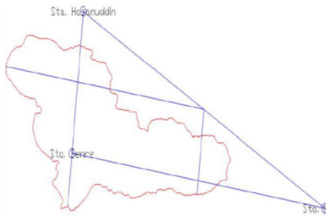
Figure 4. Thiessen's Polygon Method
