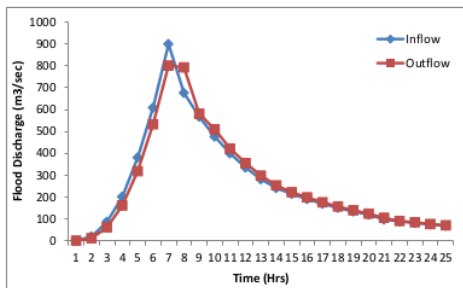
Figure 9. Flood routing for Segment 1
