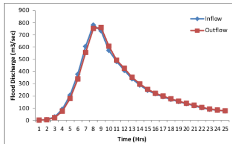
Figure 12. Flood routing for Segment 4
