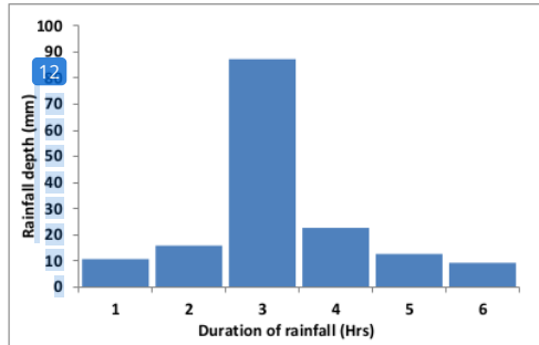
Figure 6. The hyetograph of ABM Method
