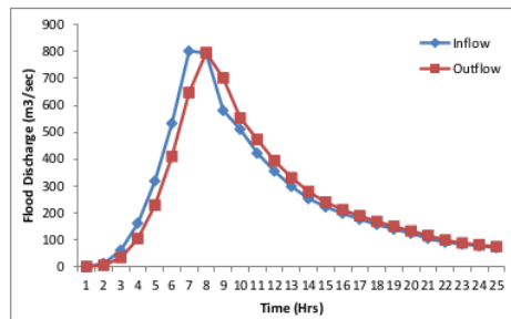
Figure 10. Flood routing for Segment 2
