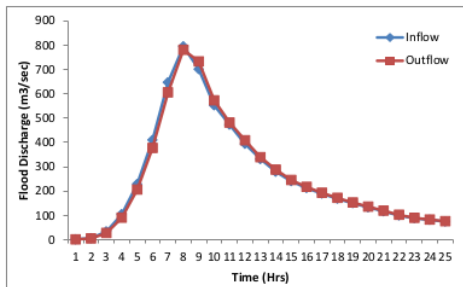
Figure 11. Flood routing for Segment 3
