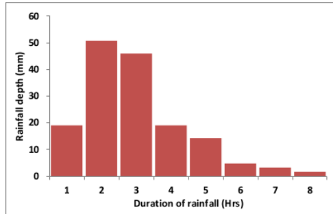
Figure 7. The hyetograph of Yusron Lubis
