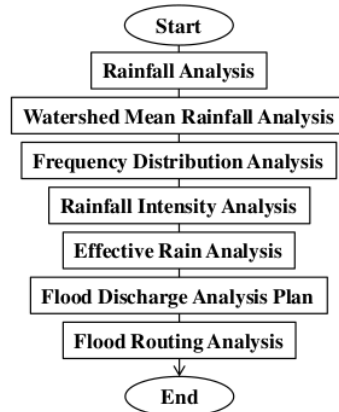
Figure 3. Flood routing analytics scheme
